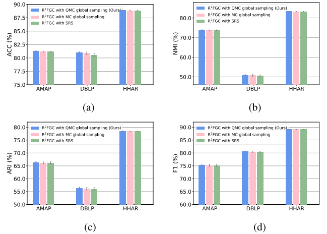
Fig. 2. Performance comparisons with respect to different global sampling strategies on the AMAP, DBLP, and HHAR datasets. (a) ACC. (b) NMI. (c) ARI. (d) F1.
